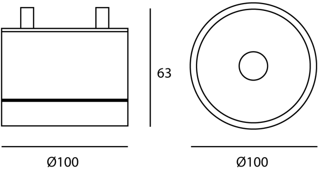
Product Dimensions
