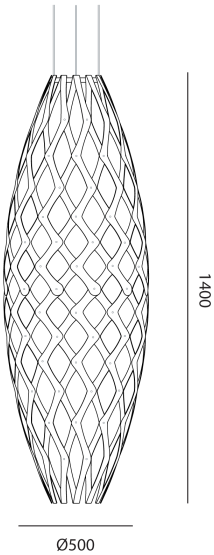
Product Dimensions
