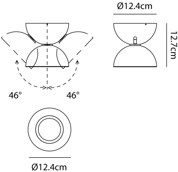
Product Dimensions
