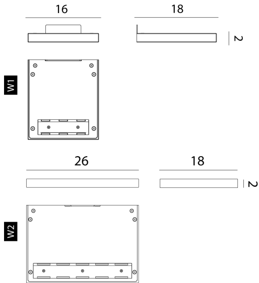
Product Dimensions
