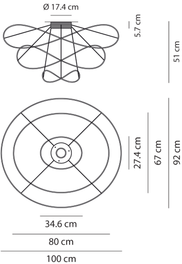
Product Dimensions
