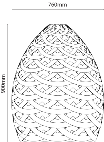
Product Dimensions
