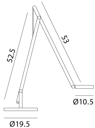
Product Dimensions
