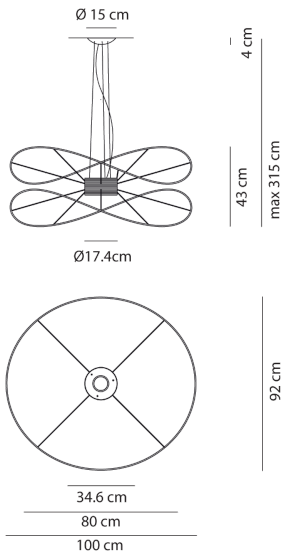
Product Dimensions
