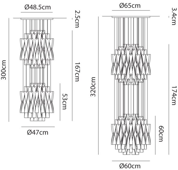
Product Dimensions
