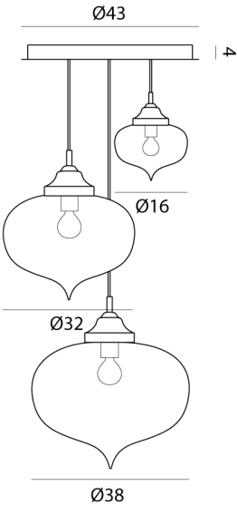
Product Dimensions
