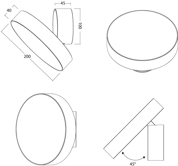
Product Dimensions
