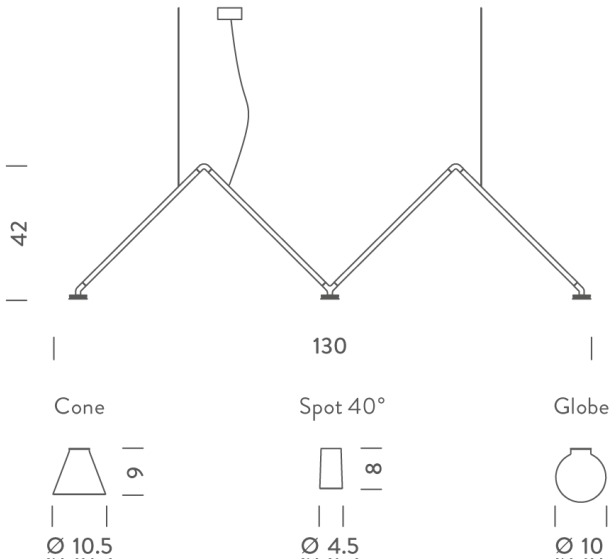
Product Dimensions
