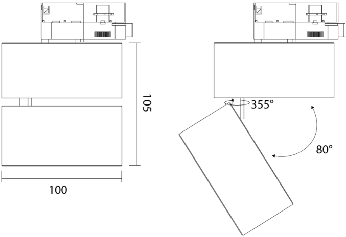
Product Dimensions
